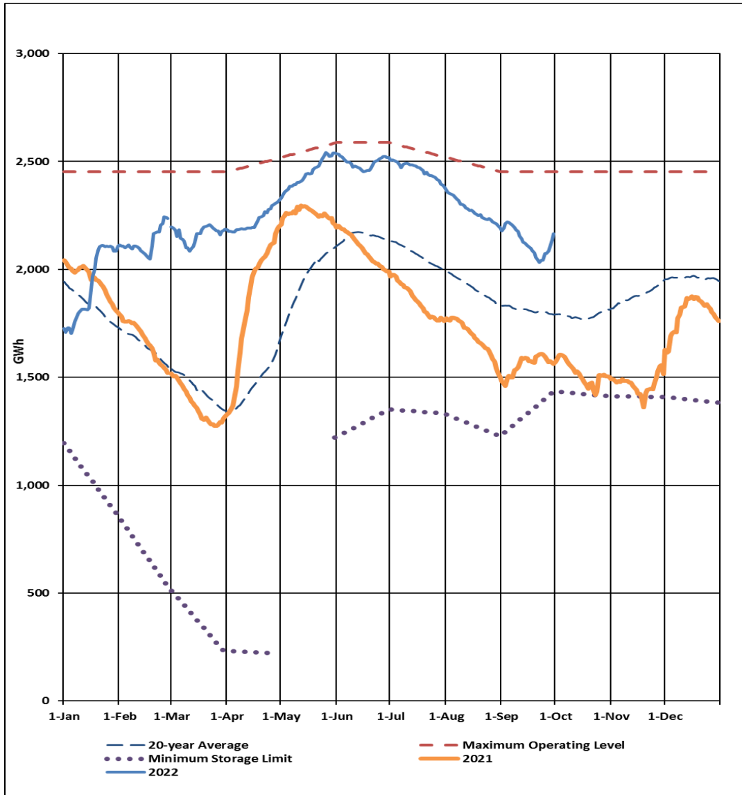
Chart 1: Total System Energy Storage for September 30, 2022
